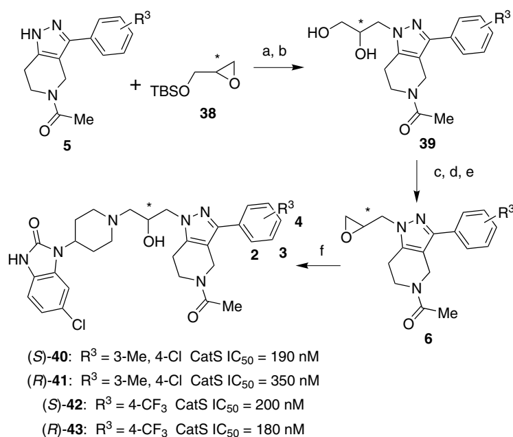
Scheme 3. Reagents and conditions: (a) \text{Cs}_2\text{CO}_3 , DMF, rt; (b) CSA, MeOH; (c) \text{MeC(OMe)}_3 , PPTS; (d) AcBr, MeOH, \text{CH}_2\text{Cl}_2 ; (e) KOEt, MeOH; (f) 6-chloro-1-piperidin-4-yl-1,3-dihydro-benzimidazol-2-one, EtOH, reflux.
