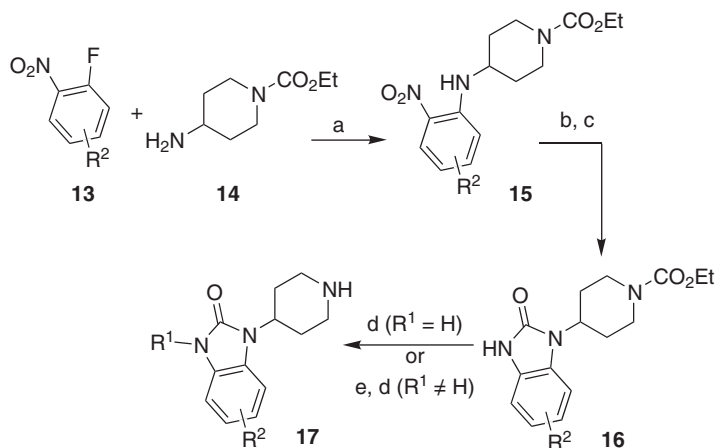
Scheme 2. Reagents and conditions: (a) DMF, 60 °C; (b) Pt/C, \text{NH}_4\text{HCO}_2 , EtOH, rt; (c) triphosgene, \text{Et}_3\text{N} , \text{CH}_2\text{Cl}_2 , rt; (d) 1 N NaOH, EtOH, reflux; (e) KHMDS, \text{R}^1\text{X} , THF.
