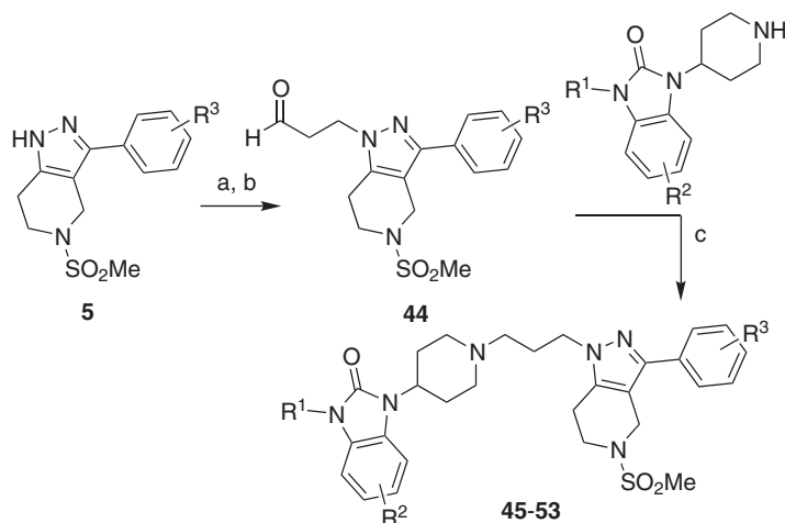
Scheme 4. Reagents and conditions: (a) 3-bromopropanol, \text{Cs}_2\text{CO}_3 , DMF; (b) Dess–Martin periodinane; (c) \text{Na(OAc)}_3\text{BH} , AcOH, \text{CH}_2\text{Cl}_2 .
