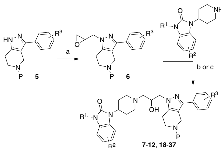
Scheme 1. Reagents and conditions: (a) epichlorohydrin (4–6 equiv), Cs 2 CO 3 (2 equiv), DMF, rt; (b) amine, 3–10% Yb(OTf) 3 , CH 2 Cl 2 , rt, 0 °C; (c) amine, EtOH, reflux.
